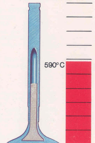
Sodium-cooled valve
