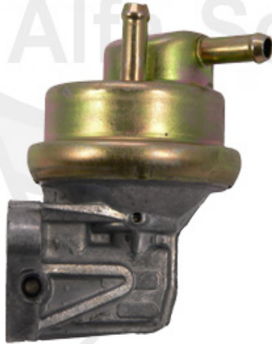
1. KP 0565 Vergaser/carburetor
